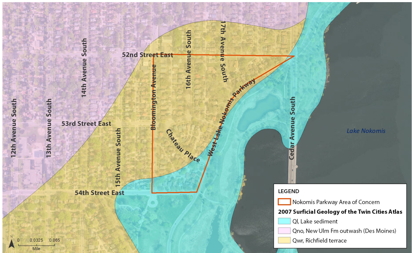
Figure 14: 2007 Surficial Geology Atlas for the Nokomis Parkway Area of Concern. Excerpt from the 2007 Surficial Geology Atlas of Hennepin County for the Nokomis Parkway Area of Concern shows homes were built over areas of lake sediment. (Credit: MCWD; Data Source: Meyer, 2007)
